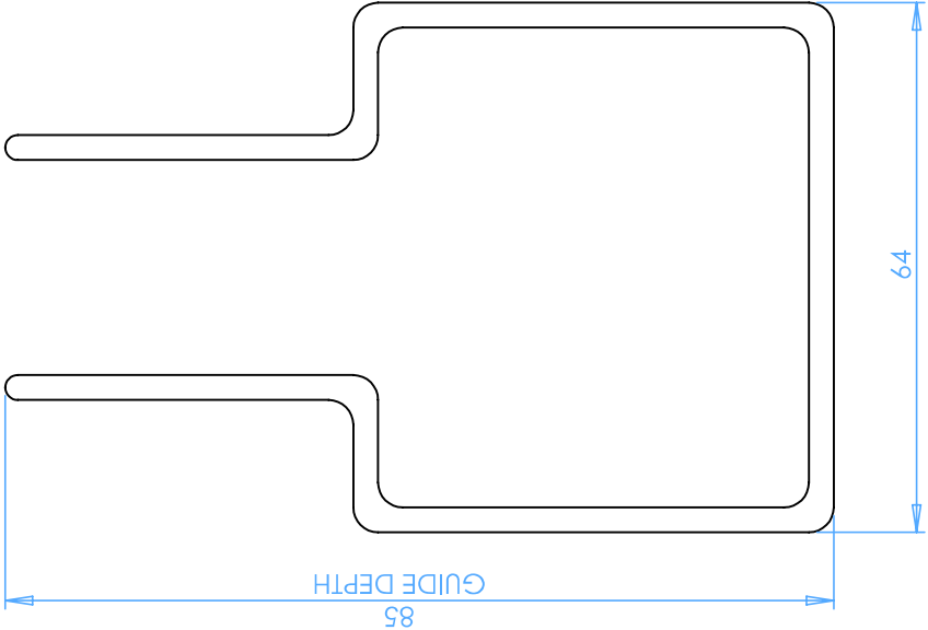
85mm WINDLOCK
